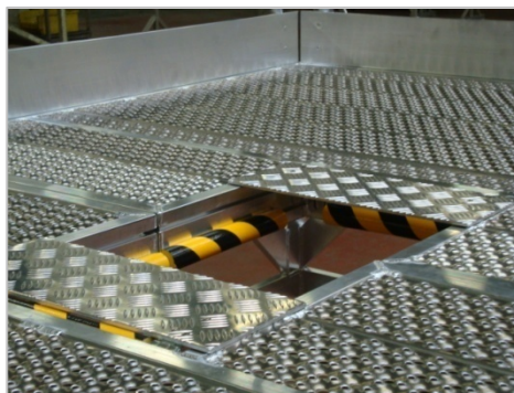
Cutout of the platform + protections designed to conform perfectly the landing gear
