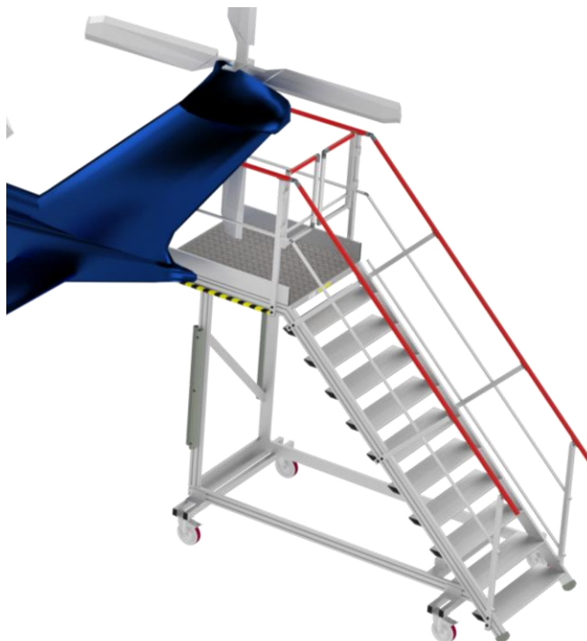
3D view staircase in use position
