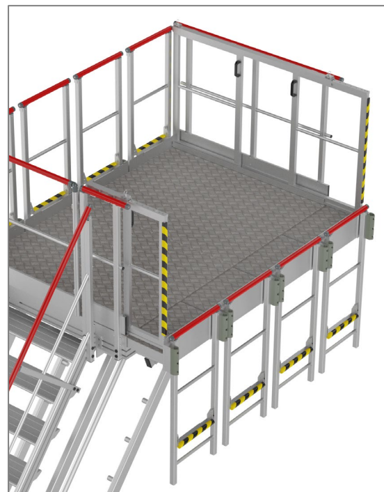
3D rear view of the stepladder
