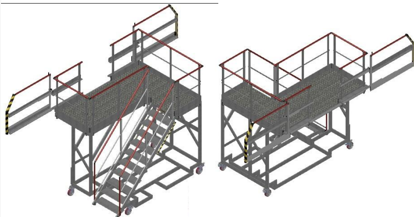
Mobile stepladder with sliding guardrails in deployed position 2 sections: one of 950 mm, the other of 550 mm – anti-shock protection
