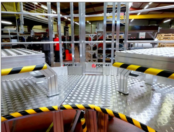
View on the down sliding bearing and swivel guardrail design to conform the shape of the two helicopter models.
