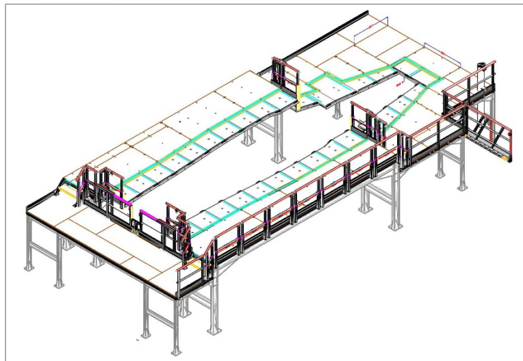
3D view of the complete platform
