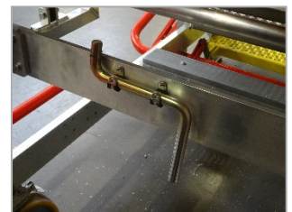
Retractable step on the rear side of the platform – Manually operated. Shockproof protection.
